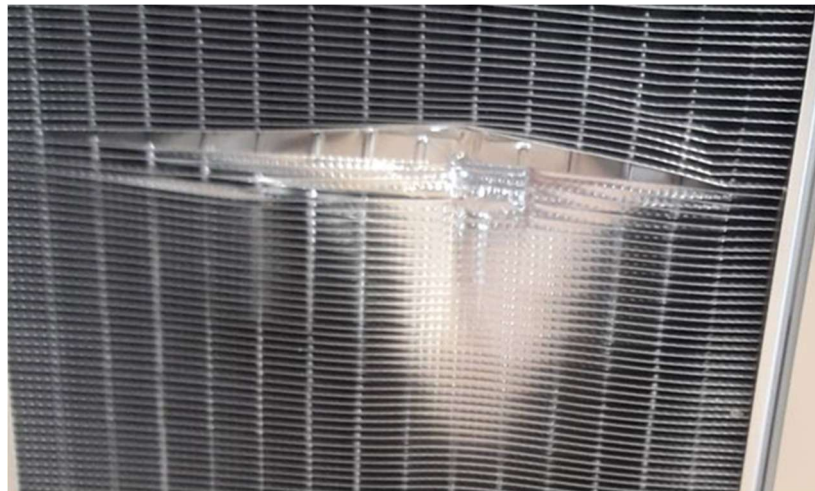
Impact damage to heat exchanger surface
