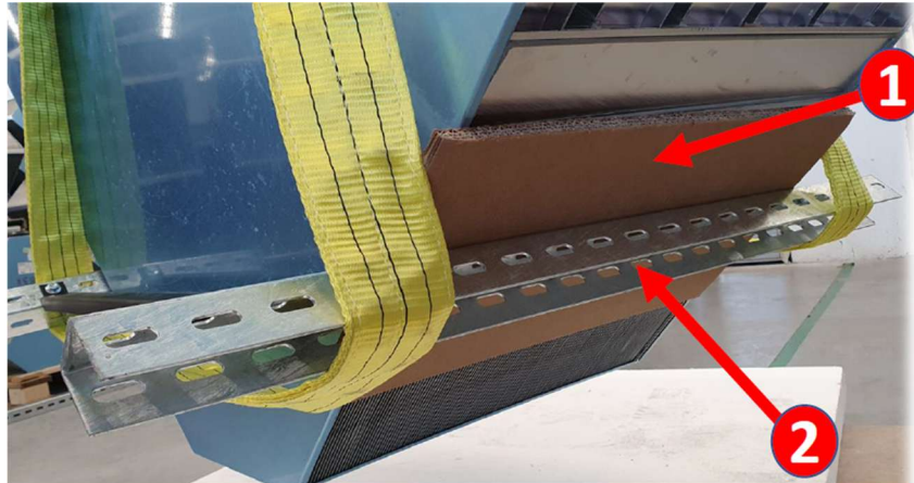
Spreader bar and slings in conjunction with packing and supporting steelwork
