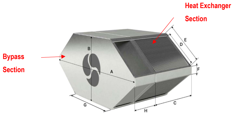
Counter flow heat exchanger
