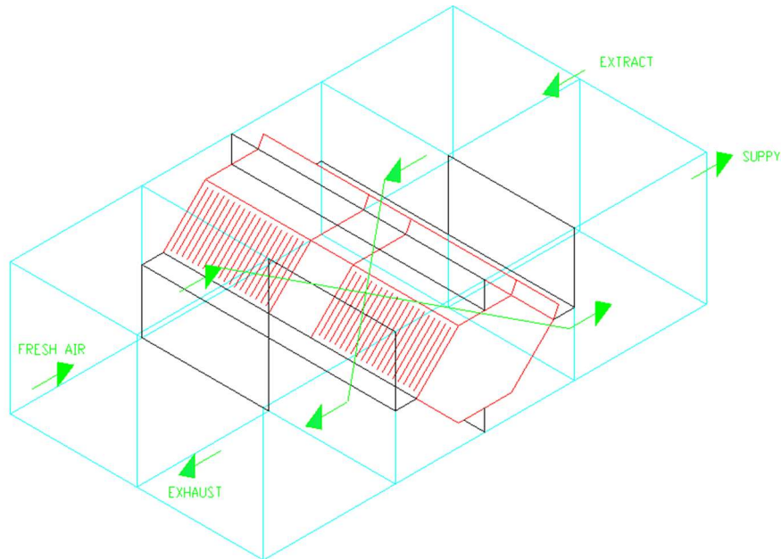
Installation of PCF counter flow plate heat exchanger in side by side AHU sections showing air flow and air dividing bulkheads
