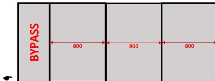
☛ C = 2400mm, Side Bypass, 3 Blocks x 800mm
