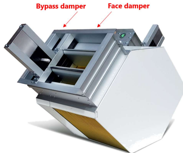
PCF-I counter flow heat exchanger with face and bypass damper
