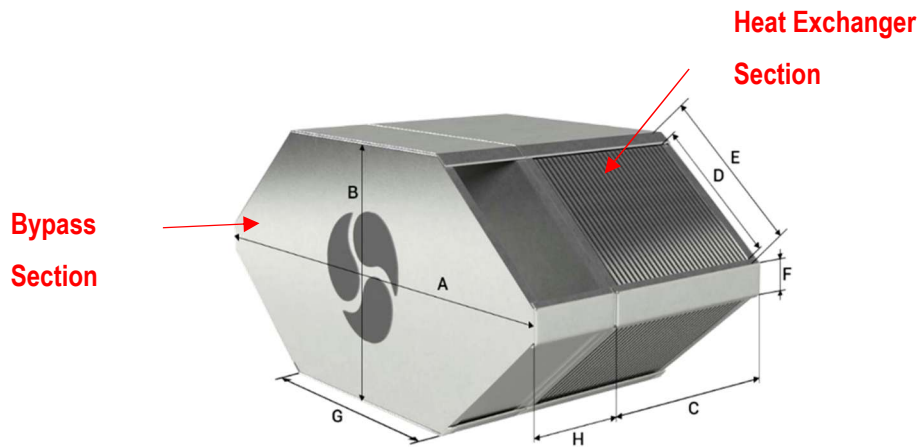
PCF counter flow heat exchanger with bypass
