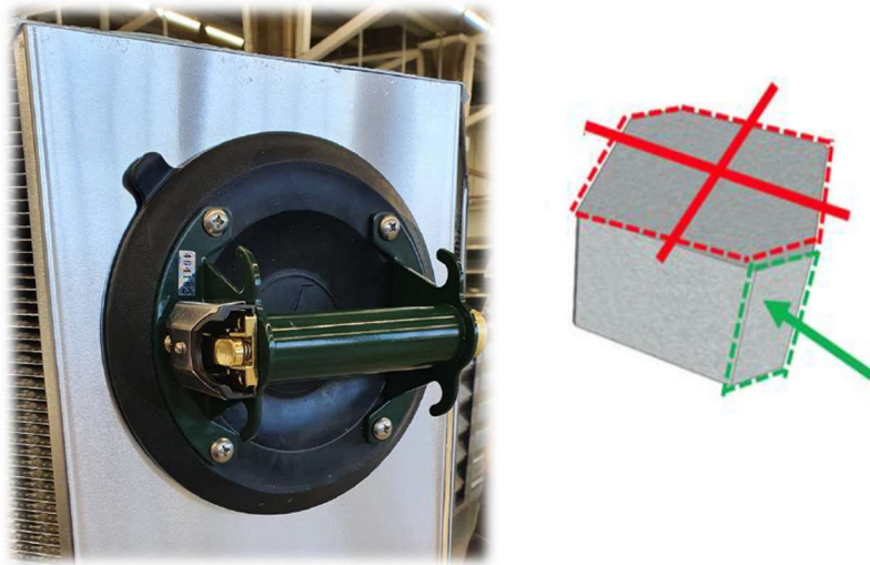
Use of vacuum grippers
