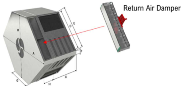
PCF-I counter flow heat exchanger with recirculation damper
